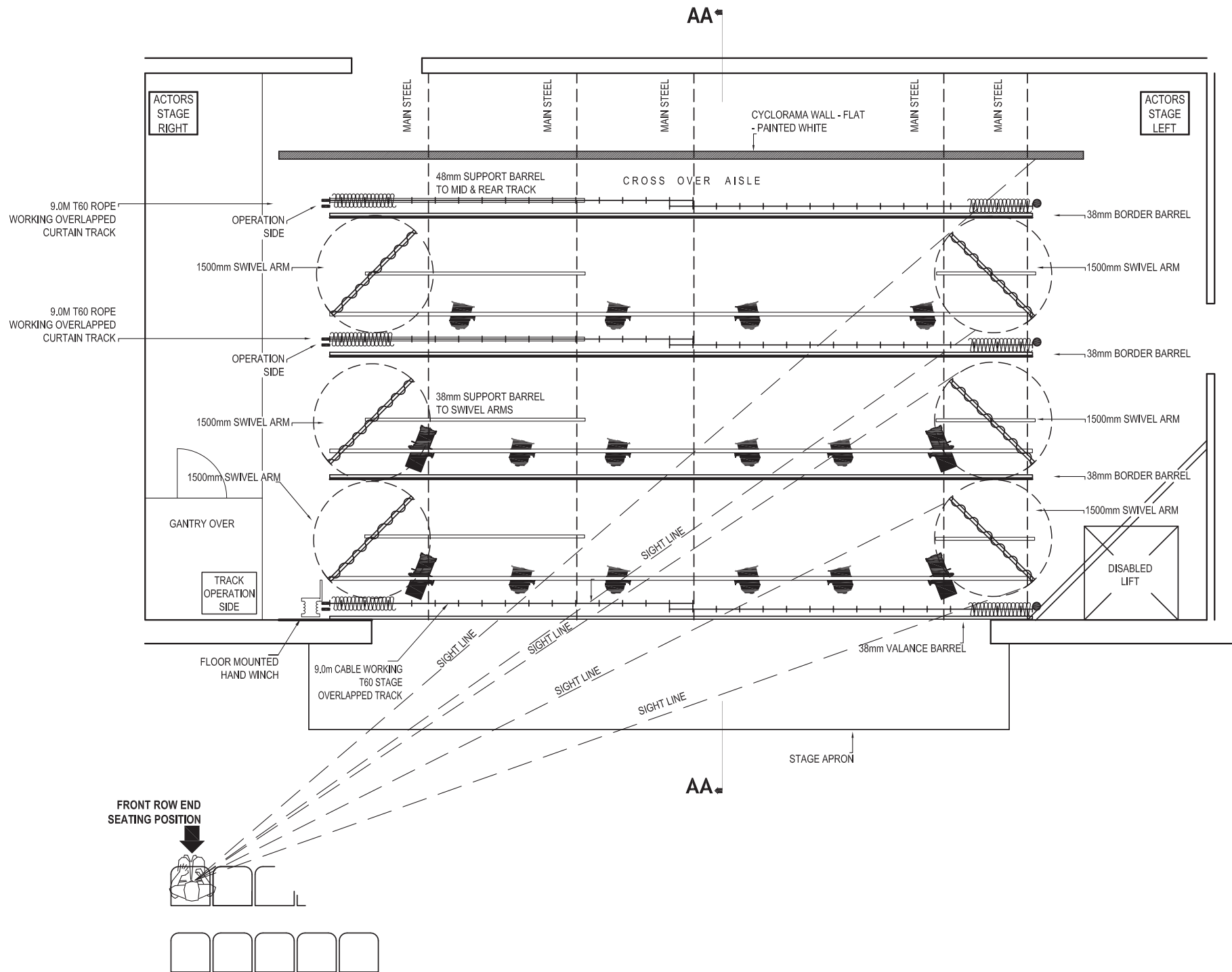
STAGE LAYOUT
